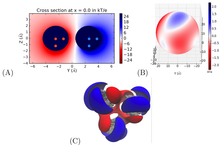
Figure 3: APBS PB-AM electrostatic potential results for (A) 2D cross section for the electrostatic potential outside of two collections of point charges (each with net charge \pm 6 , charge positions indicated by red and blue circles), (B) potential on the spherical coarse-grain surface of a barstar molecule, (C) VMD [66] of the transmembrane trimer Omp32 porin (molecules are given in gray and isosurfaces are drawn at 1.0 (blue) and -1.0 (red)). All calculations were performed at 0.0 M ionic strength, pH 7, protein dielectric 2, and solvent dielectric 78. All electrostatic potentials are given in units of kT/e .
