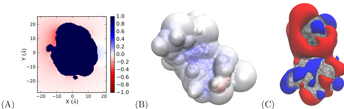
Figure 4: APBS PB-SAM electrostatic potential results for (A) potential in a 2D plane surrounding the barstar molecule, (B) potential over range [-1, 1] on the coarse-grain surface of the barnase molecule (blue region is the location of barstar association, (C) VMD [66] visualization of the ESP around the association of barnase and barstar (molecules are given in gray and isosurfaces are drawn at 1.0 (blue) and -1.0 (red)). All calculations were performed at 0.0 M ionic strength, pH 7, protein dielectric 2, and solvent dielectric 78. All electrostatic potentials are given in units of kT/e .
