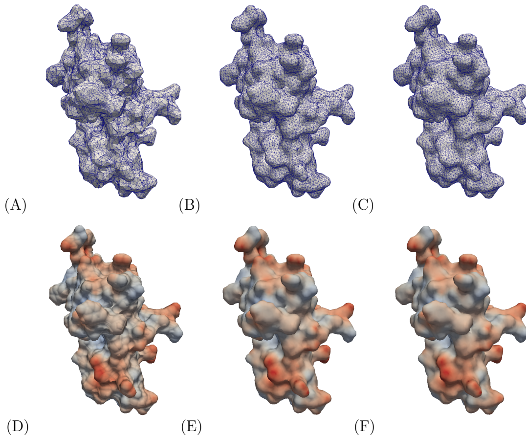
Figure 2: APBS TABI-PB electrostatic potential results for PDB ID 1a63. Surfaces were generated with (A) 20228 triangles via MSMS [62], (B) 20744 triangles via NanoShaper SES, and (C) 21084 triangles via NanoShaper Skin [63]. These discretizations resulted in surface potentials (with units kT/e ) of (D) MSMS in range [-8.7, 8.6] , (E) NanoShaper SES in range [-13.4, 7.5] , and (F) NanoShaper Skin in range [-33.8, 8.0] . All calculations were performed at 0.15 M ionic strength in 1:1 salt, with protein dielectric 1, solvent dielectric 80, and temperature 300K.
