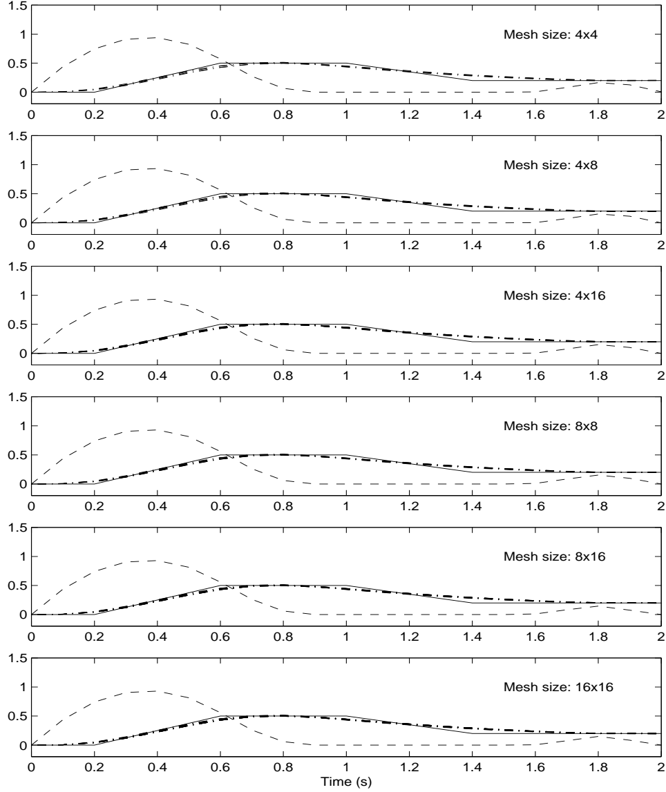
Fig. 1. Optimal solutions for increasing mesh size. Solid line: \tau(t) . Dashed line: u(t) . Dash-dot lines: T_{ij}(t) in \Omega_c .
